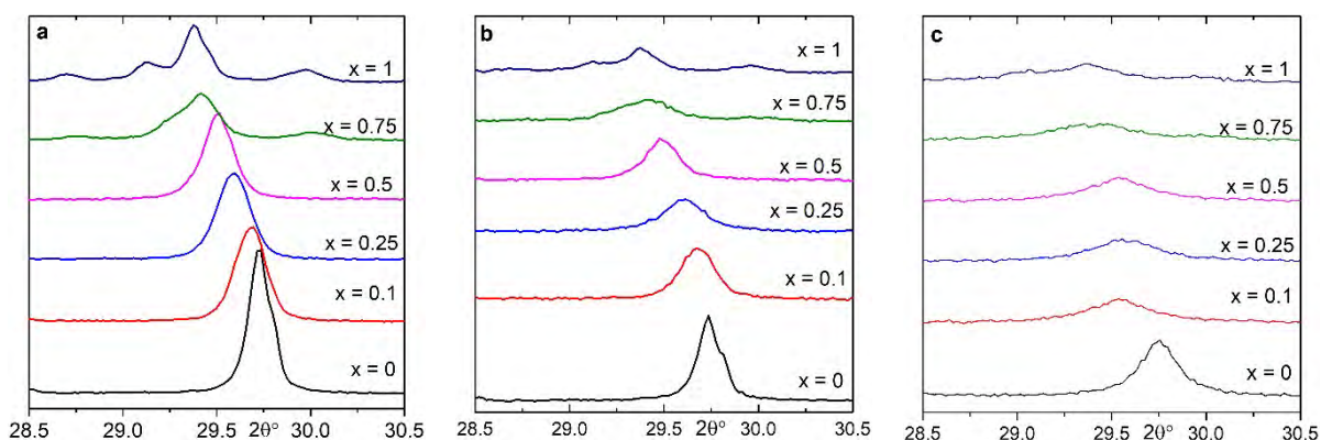
Figure 1. Comparison of XRD patterns of \text{Ag}_{7+x}(\text{P}_{1-x}\text{Si}_x)\text{S}_6 solid solution in form of microcrystalline (a) and nanopowders grinded for 30 (b) and 60 (c) min.
