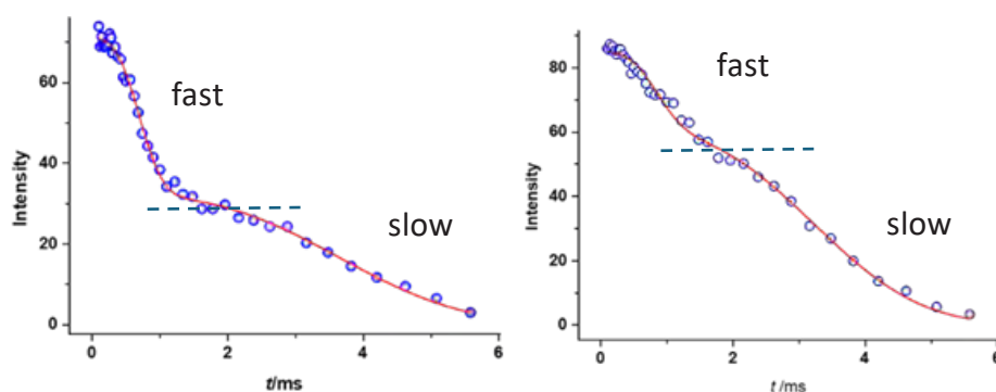
Figure 1. The Hahn-echo profile of a 70 years (left) and 25 years (right) old male person.
