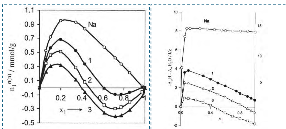
Figure 1. Left: Adsorption excess isotherms for Na + illite (Na) and hexadecylpyridinium illites (1,2,3: increasing amounts of hexadecylpyridinium ions) in methanol(1)-benzene(2). Right: the corresponding immersional wetting enthalpy isotherms.
