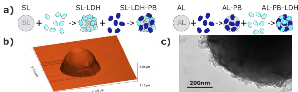
Figure 1. a) Schematic illustration of the nanozyme immobilization steps, b) AFM-in-SEM and c) TEM image of a LDH-covered SL particle.
