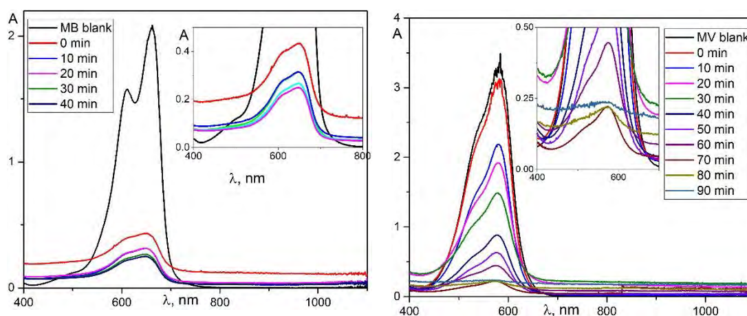
Figure 1. Absorption spectra of the \text{LaFe}_{0.95}\text{Cu}_{0.05}\text{O}_3 + MB (a) and \text{LaFe}_{0.95}\text{Cu}_{0.05}\text{O}_3 + MV (b) mixtures.
