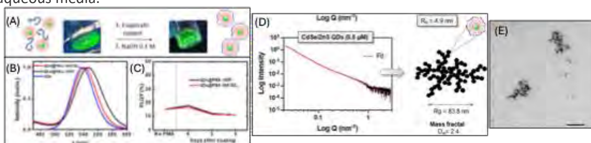
Figure 1. (A) Representation of the polymer coating process of QDs; (B) Photoluminescence of QDs; (C) PLQY of polymer-coated QDs; (D) SAXS analysis of fractal arrangements; (E) TEM micrograph of polymer-coated QDs (scale bar 100 nm).
